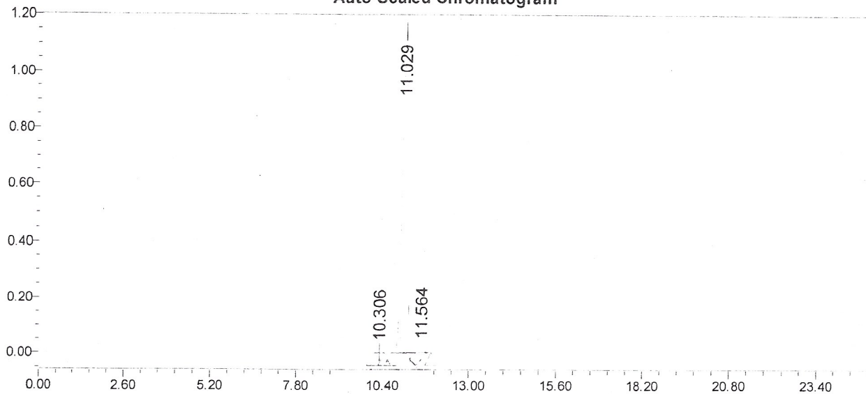
Auto-Scaled Chromatogram
